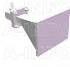
LB-90-15-C-TFSP0 Standard Gain Horn Antenna 8.2-12.4GHz 15dB Gain TNC Female
